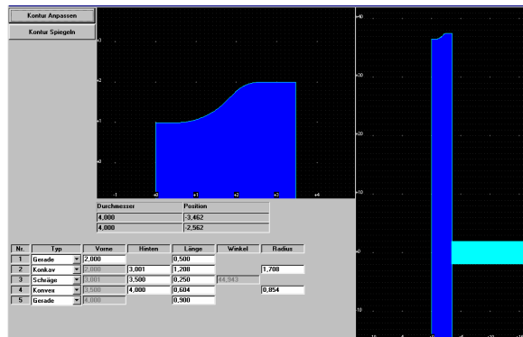
Wheel Construction
